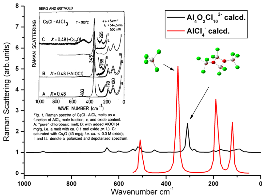
Figure. Example of experimental Raman spectra of CsCl-AlCl 3 melts with oxygen contaminations and new model calculated structures and spectra. The experimental data are from ref. [2].
